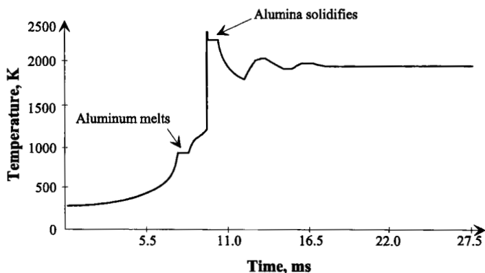
FIG. 22. Temperature-time profile of a single cell for the TiO 2 -Al-C reaction (Adapted from Bowen and Derby, 1993).
