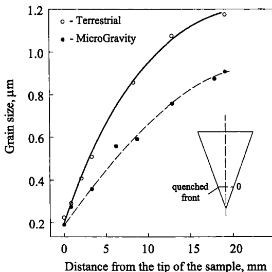
FIG. 58. Evolution of \text{TiB}_2 (dark phase) grain size in \text{Ni}_3\text{Al} (bright phase) matrix during combustion synthesis in the (Ti-2B)-(3Ni-Al) system (Adapted from Mukasyan et al. , 1997b).
