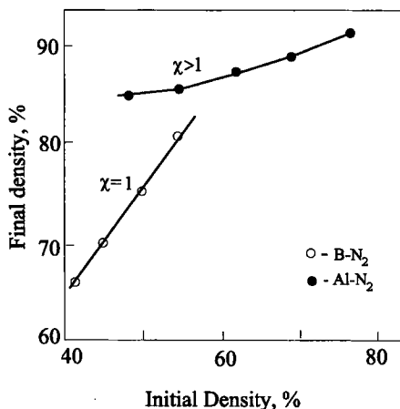
FIG. 46. Final sample density as a function of initial density for B-N 2 (Mukasyan, 1986) and Al-N 2 (Dunnead et al. , 1990a) systems.
