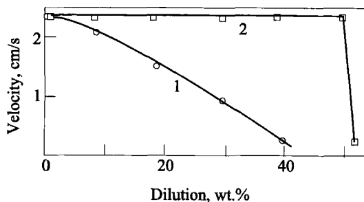
FIG. 37. Combustion velocity as a function of inert dilution: curve 1, d_{\text{TiC}} = 50\text{--}90 nm; curve 2, d_{\text{TiC}} = 1000\text{--}1500 nm (Adapted from Maslov et al. , 1990).
