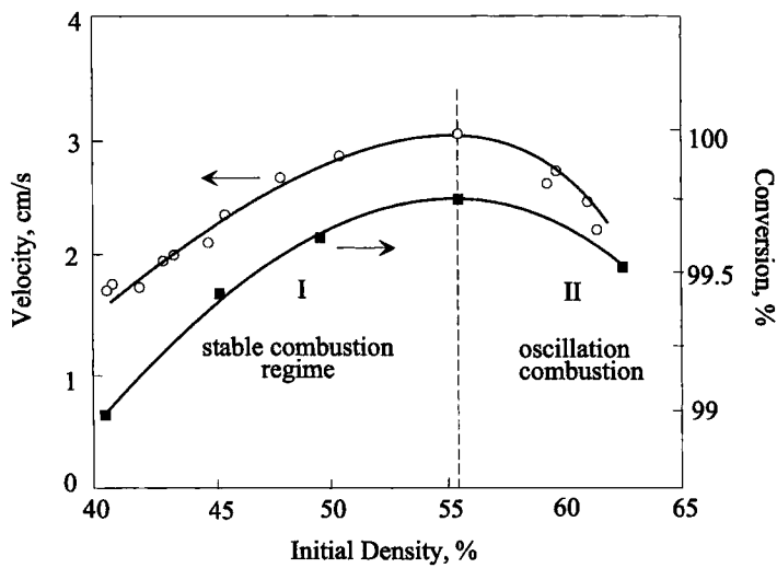
FIG. 42. The dependences of combustion velocity and conversion on initial sample density in Ti-C system (Adapted from Shkiro and Borovinskaya, 1975).
