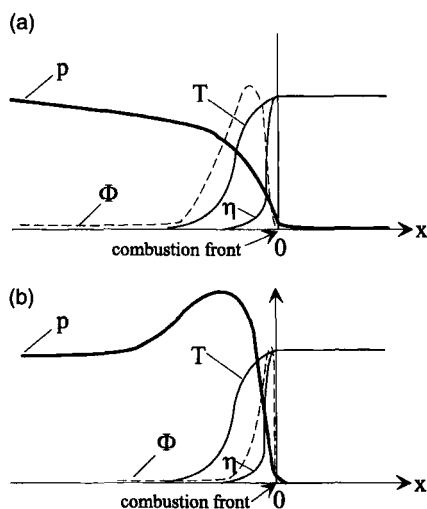
FIG. 28. Gas pressure ( p ), temperature ( T ), conversion ( \eta ), and heat release function ( \Phi ) distributions in the combustion front: (a) L_f/L_f^{cr} > 1 ; (b) L_f/L_f^{cr} < 1 (Adapted from Aldushin et al. , 1976b).
