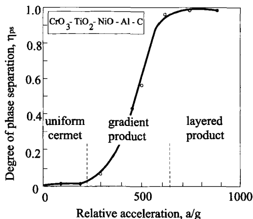
FIG. 10. The degree of phase separation as a function of centrifugal acceleration, a , where g is acceleration due to gravity (Adapted from Merzhanov and Yuhvid, 1990).
