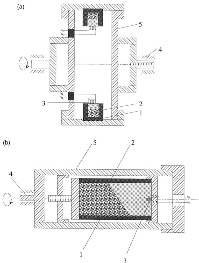
FIG. 9. Scheme of SHS+centrifugal casting: (a) radial centrifuge; (b) axial centrifuge. 1-sample container; 2-reactant mixture; 3-ignitor; 4-axle; 5-reactor. (Adapted from Merzhanov and Yuhvid, 1990)
