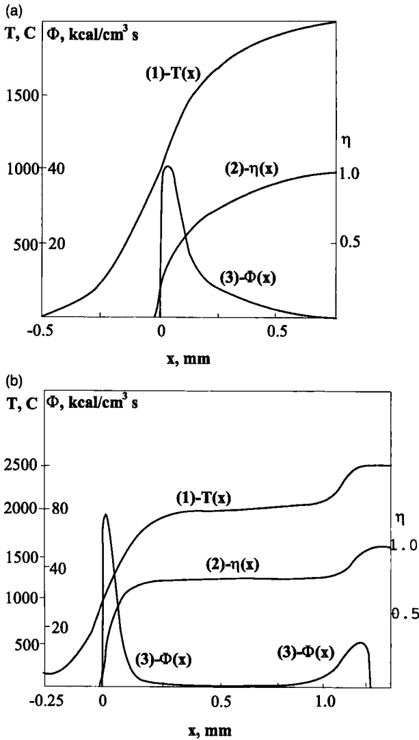
FIG. 71. Average temperature distribution over the combustion zones of the mixture Nb+xB , rate of heat release \Phi , and degree of conversion, \eta : (a) the mixture Nb+2B ; (b) Nb+B (Adapted from Zenin et al. , 1980).
